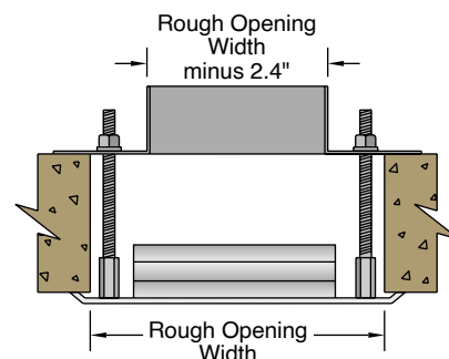
TOP SECTION
