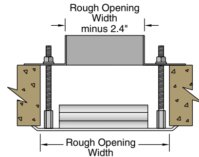
TOP SECTION
