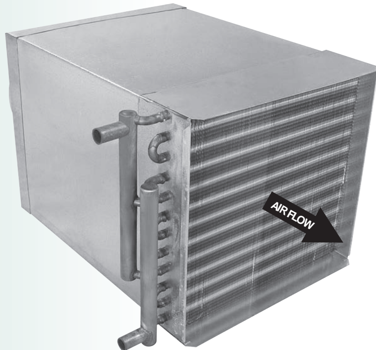
Model EZT Single Duct with 2 row hot water coil, right hand header connections
