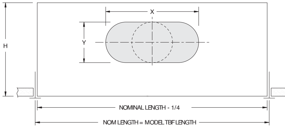
VIEW FROM INLET SIDE
