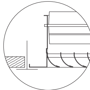
45° DEFECTION, 3/4" (19) SPACING
