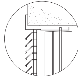
45° DEFECTION, 1/2" (13) SPACING
