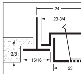
Model PDX-T Tegular, 15/16" (shown)
