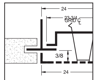
Model PDX-C Concealed Spline
