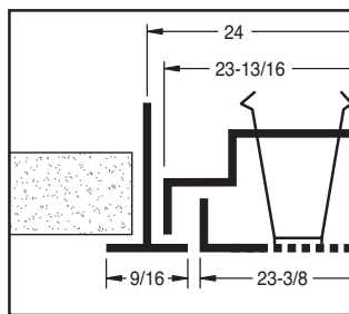
Model PDX-L9 Lay-In, 9/16"
