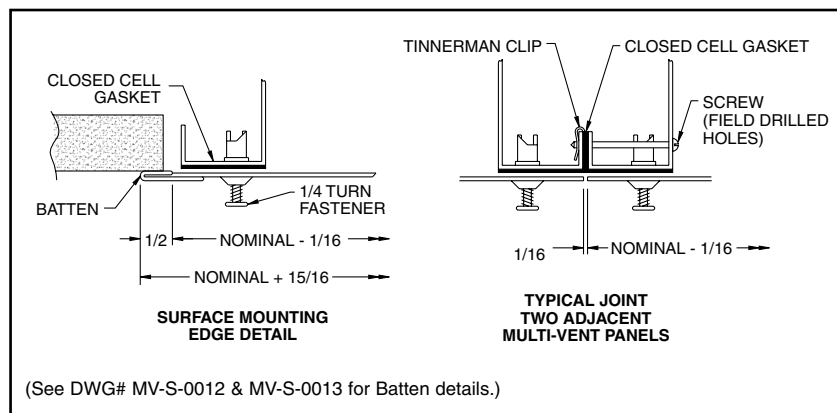
Model MV-1P Surface Mounted
