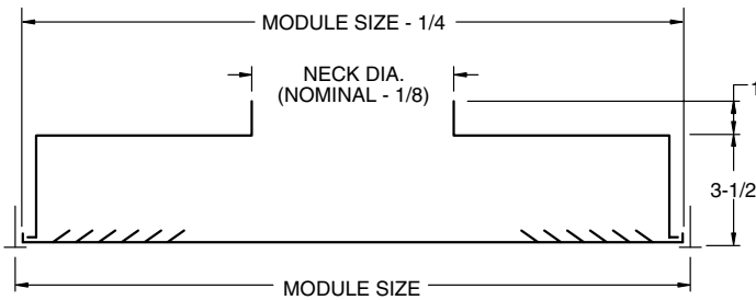
Model MVAT - Lay-In T-Bar
