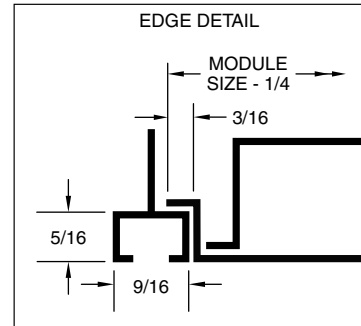
Model MVAD - 9/16" Narrow Slot
