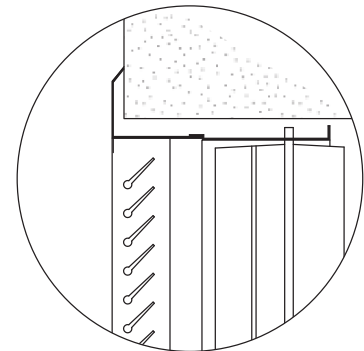
40° DEFECTION, 1/2" SPACING
