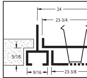
Model 3PD-D 9/16" NARROW SLOT
