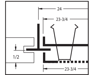
Model 3PD-V VECTOR CEILING *
