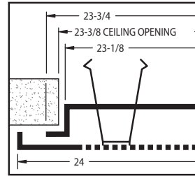
Model 3PD-F SURFACE MOUNTED
