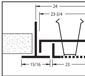
Model 3PD-L Lay-In, 15/16" (shown)
