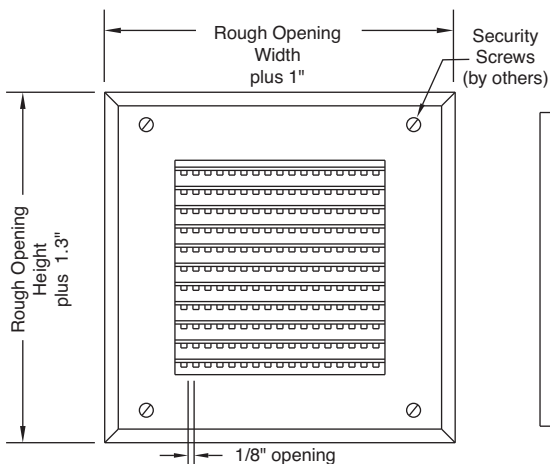
FRONT SECTION
