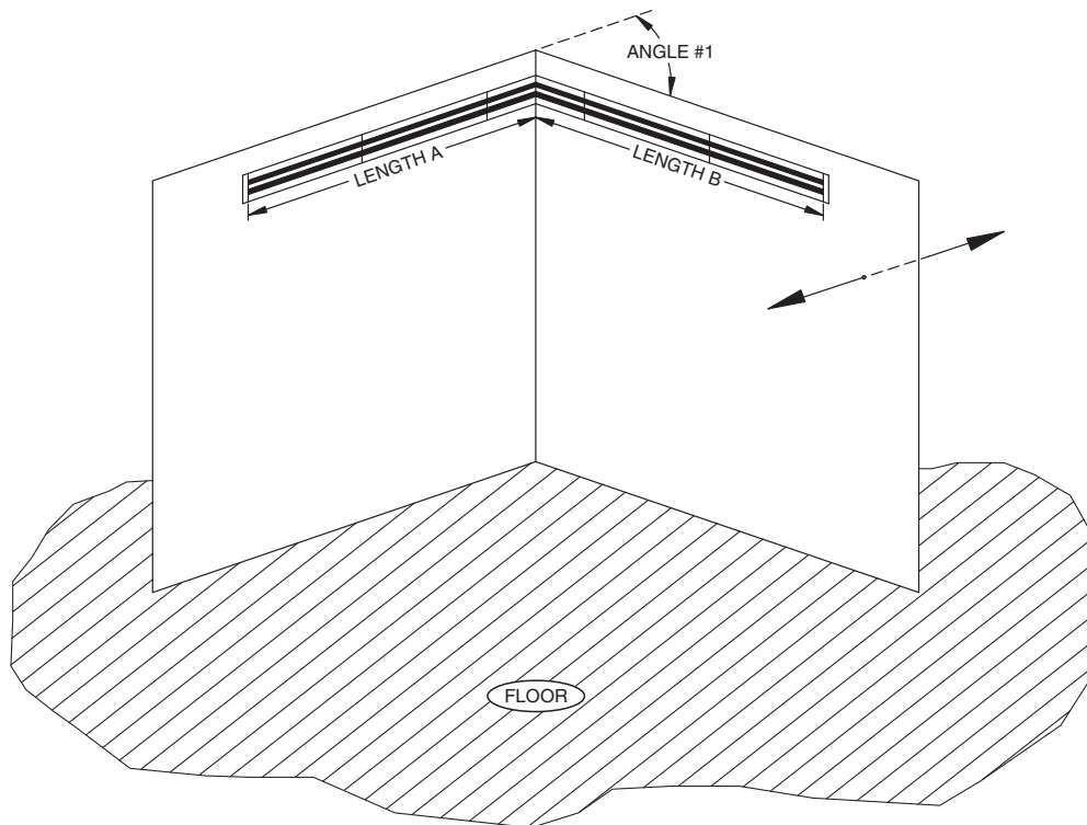
DETAIL A
