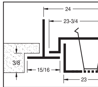
Model CG-T Tegular, 15/16" (shown)
