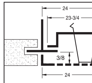
Model CG-C Concealed Spline
