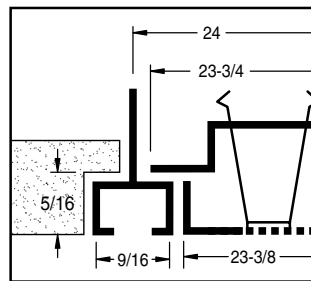
Model CG-D 9/16" NARROW SLOT
