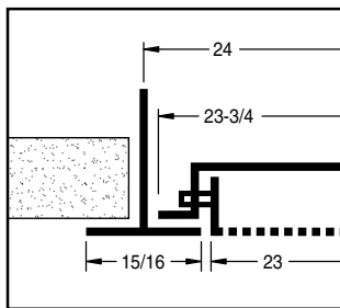
Model CG-L Lay-In, 15/16" (shown)
