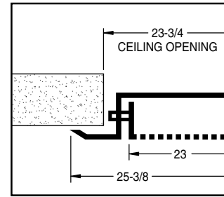
Model CG-F SURFACE MOUNTED
