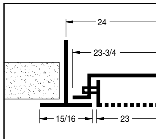
Model PDX-L Lay-In, 15/16" (shown)
