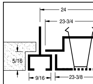
Model PDX-D 9/16" NARROW SLOT
