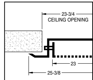
Model PDX-F SURFACE MOUNTED
