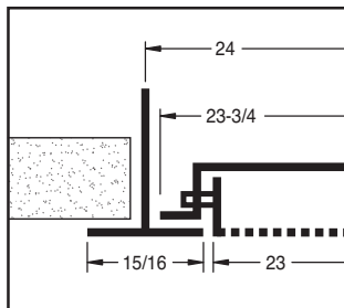
Model PD-L Lay-In, 15/16" (shown)
