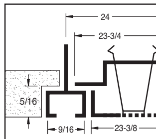
Model PD-D 9/16" NARROW SLOT
