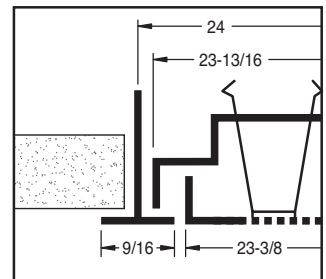
Model PD-L9 Lay-In, 9/16"
