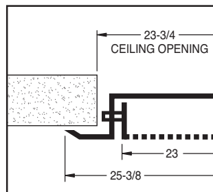
Model PD-F SURFACE MOUNTED
