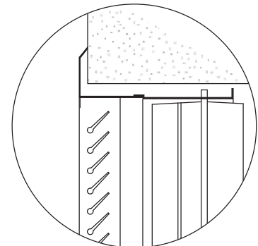
40° DEFECTION, 1/2" SPACING
