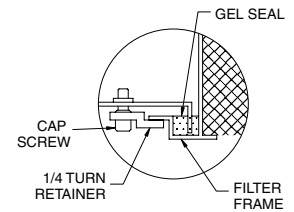
FILTER GEL SEAL EDGE DETAIL
