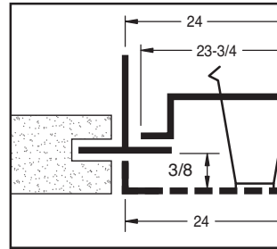
Model 3PD-C Concealed Spline
