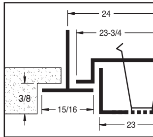
Model 3PD-T Tegular, 15/16" (shown)
